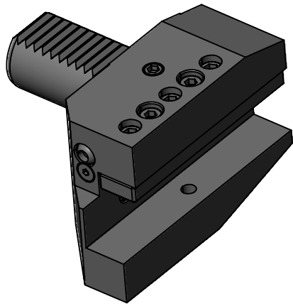
90DEG VDI30 STATIC TOOL OUTPUT: 20mm SQR SHANK COOLANT: EXTERNAL
